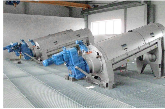
HUBER Screw Press units for sludge treatment – best dewatering performance and highest volume reduction for lower disposal costs.
