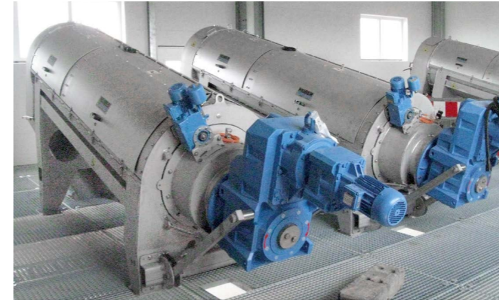
HUBER Screw Press units for sludge treatment – best dewatering performance and highest volume reduction for lower disposal costs.
