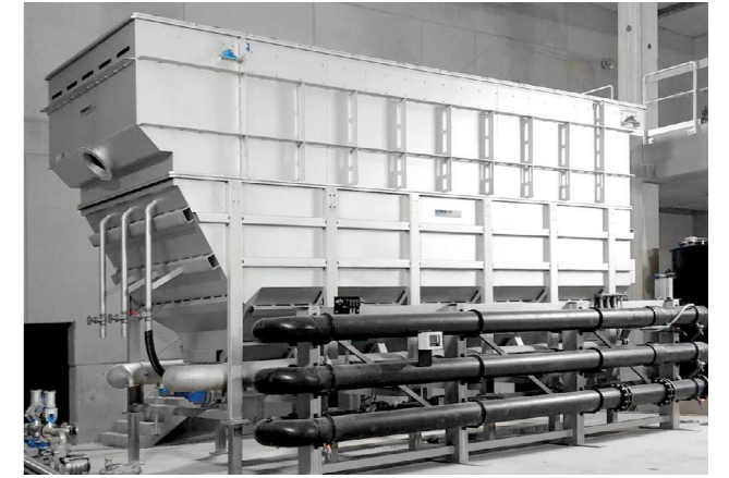
HUBER Dissolved Air Flotation for physical-chemical pre-treatment – optimum reduction of COD, fats and solids, more than 500 installations worldwide.
